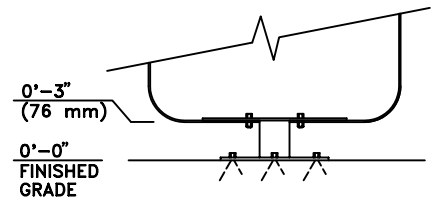
2817-DT-P (PEDESTAL MOUNT) SCALE: 3/4"=1'-0"
