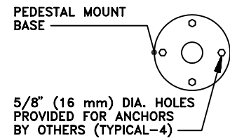
2817-DT-E (EMBEDMENT) SCALE: 3/4"=1'-0"
